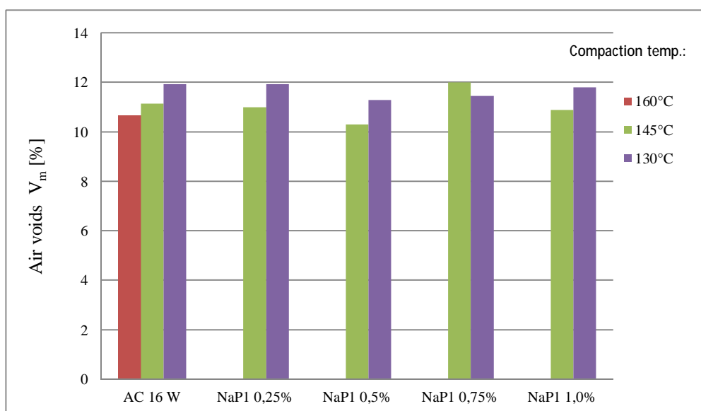
Fig. 9. Compactibility AC with zeolite material type Na-P1
